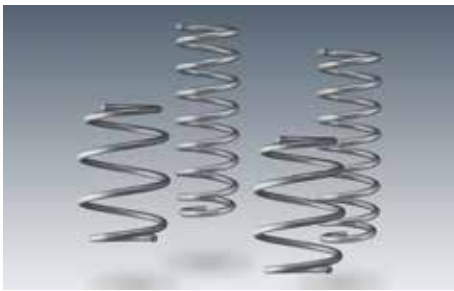
Spring kit, lowering front approx.: 25 mm rear approx.: 20 mm
